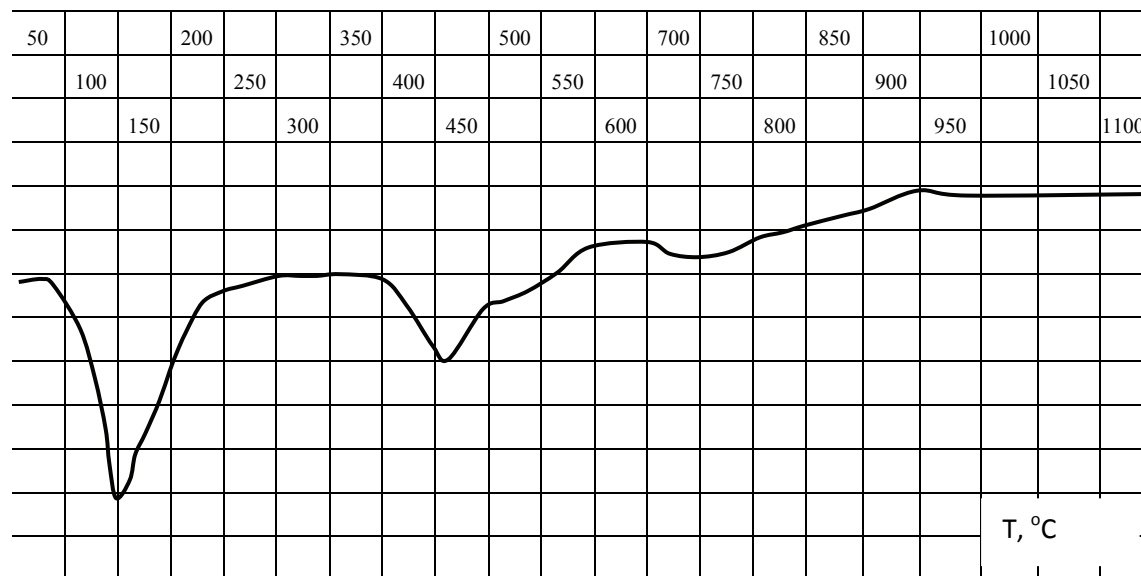
FIGURE 2. DTA raw mix with the addition of 70 wt. parts of BTPP ash and 5 wt. parts of Portland cement
