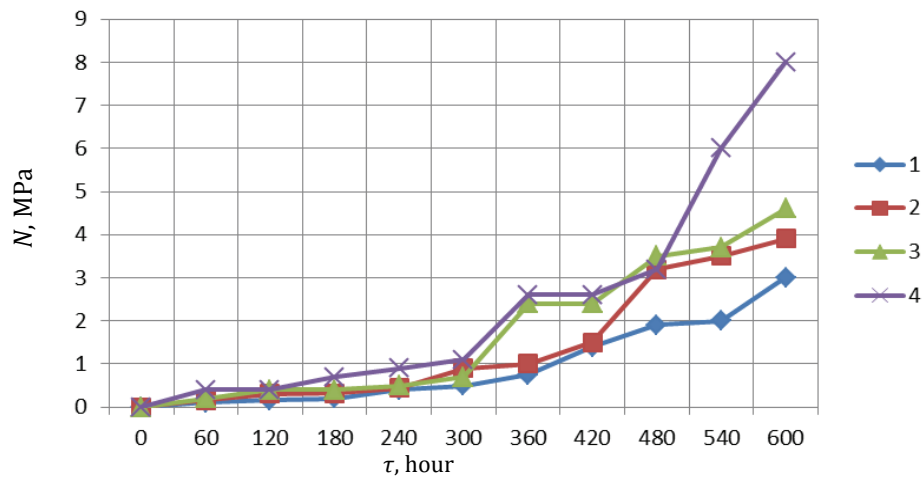
FIGURE 3. The strength of the aerated concrete arrays, depending on the type of raw material mixture: 1 – cement-sand aerated concrete, 2 – cement-ash aerated concrete, 3 – cement-ash aerated concrete with the addition of sodium sulphate (1%), 4 – cement-ash aerated concrete with the addition of sodium chloride (1%)
